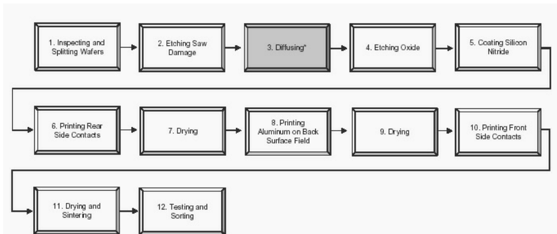
Solar Cell Manufacturing Process Flow Chart
