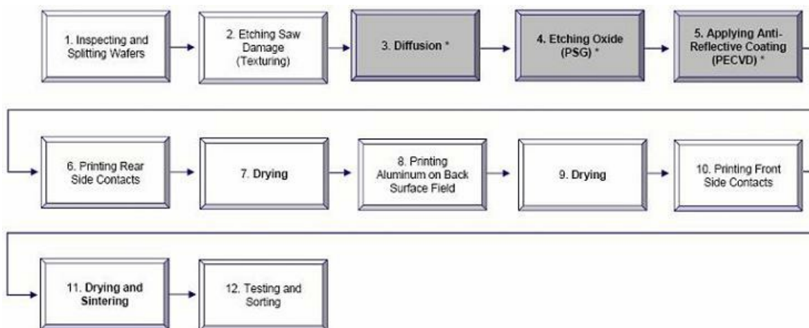
Solar Cell Manufacturing Process Flow Chart
